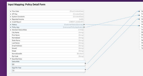
Graphical Data Editors
